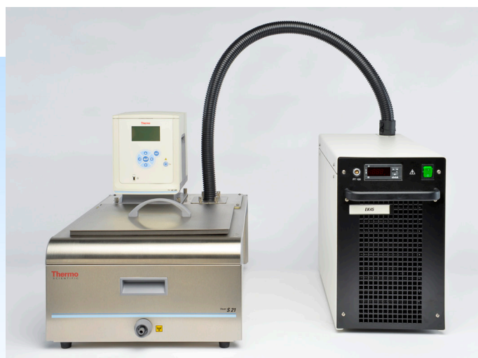
Thermo Scientific™ EK45 Immersion Cooler with a SAHARA S21 Stainless-Steel Heated Bath Circulator
